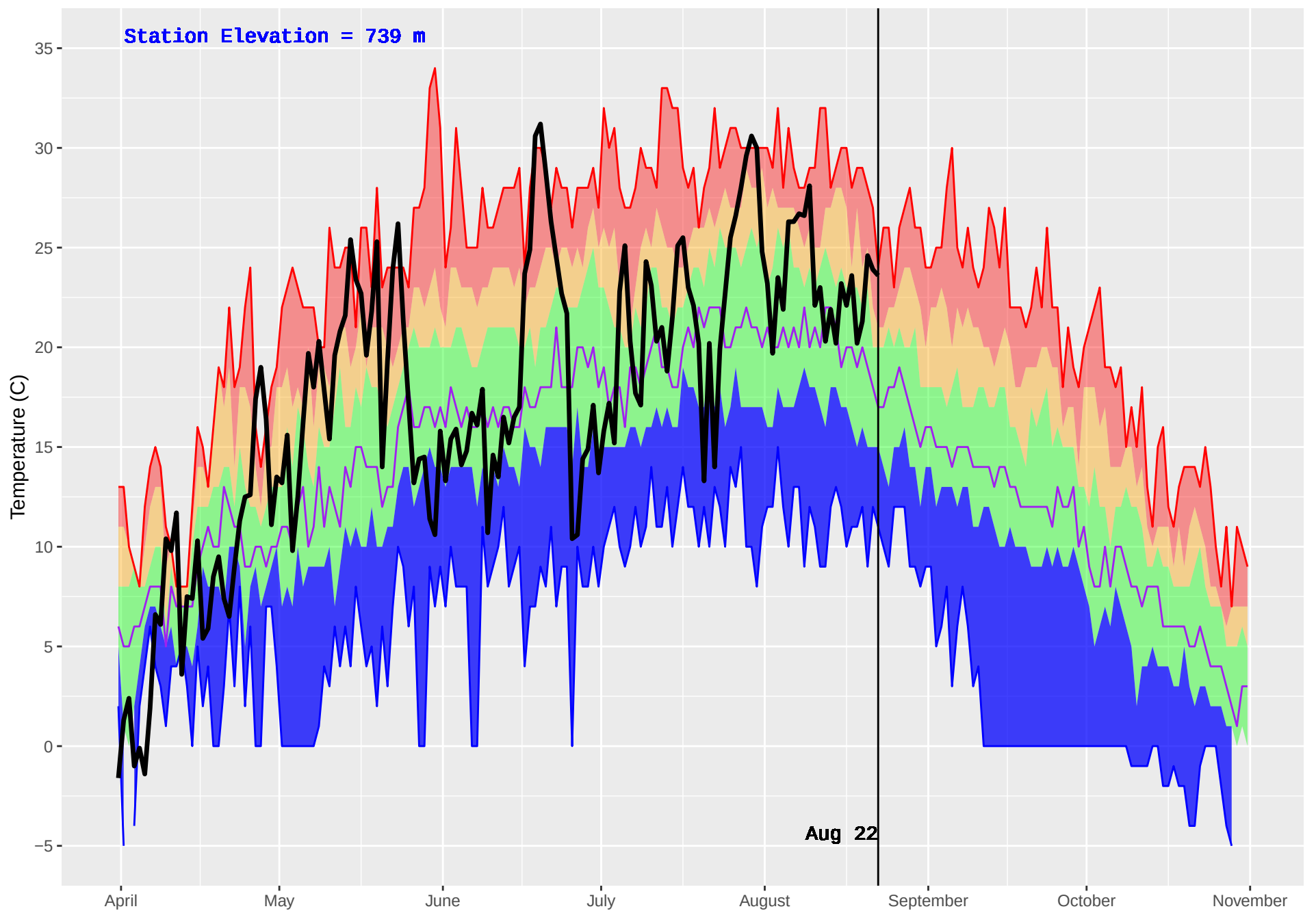
BEAR LAKE (149) : Historical (1980–2016) and Current (2018) Daily Temperature
